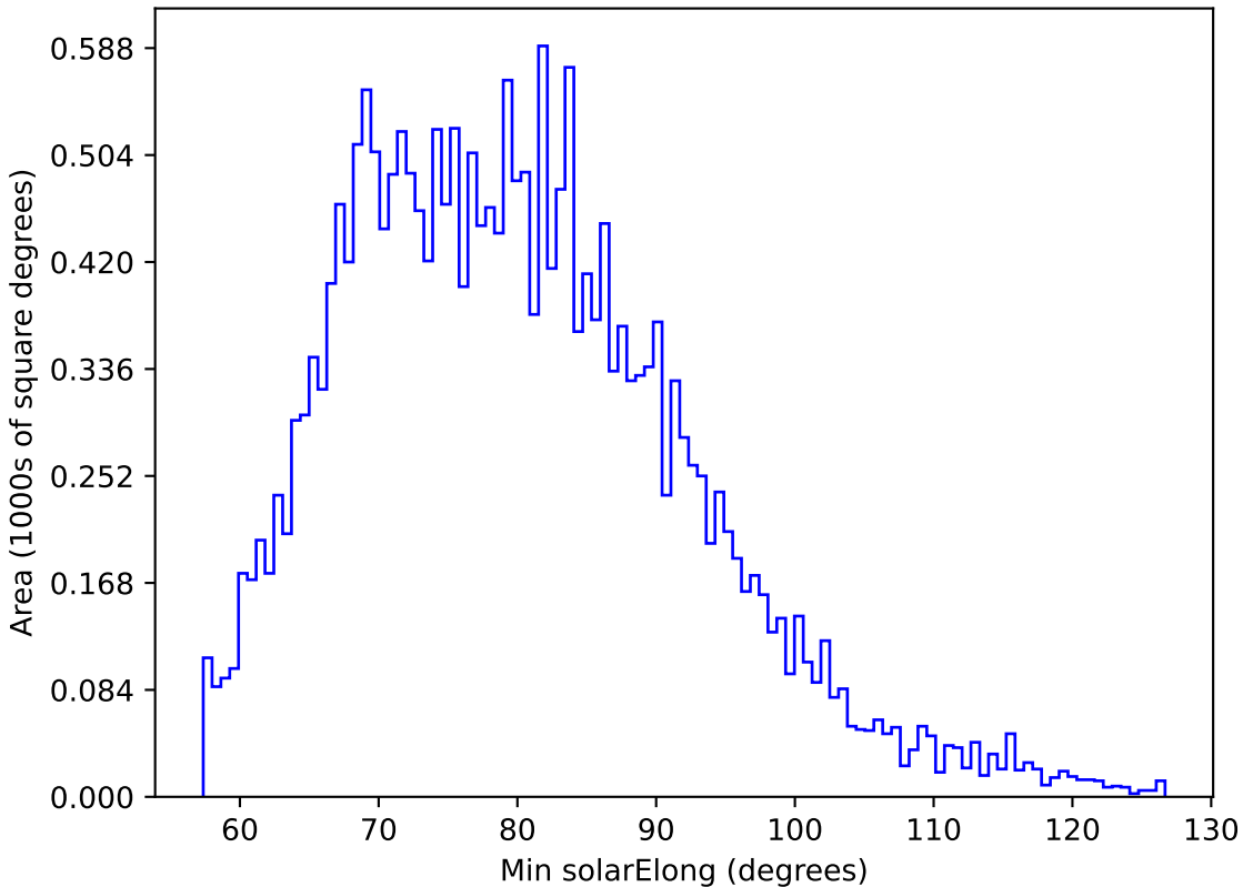
ddf_loaded_fl4_v3.4_10yrs All sky u band: Min solarElong
