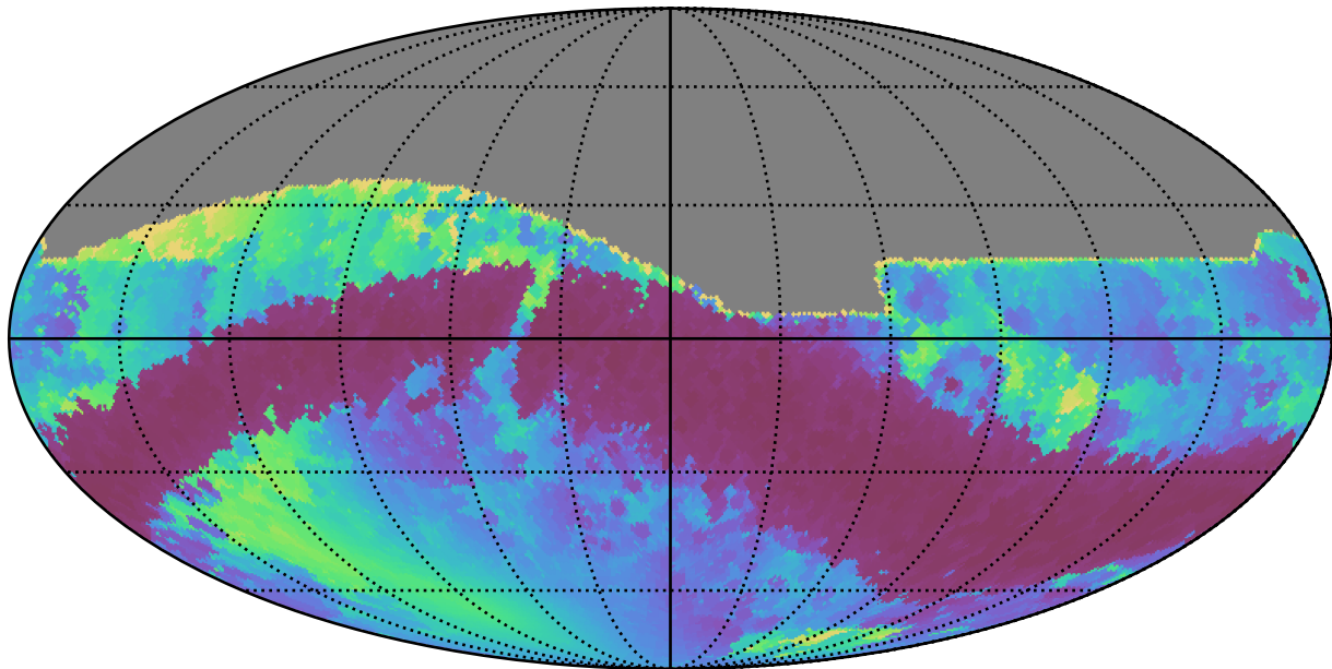
ddf_loaded_fl4_v3.4_10yrs All sky r band: Min solarElong
