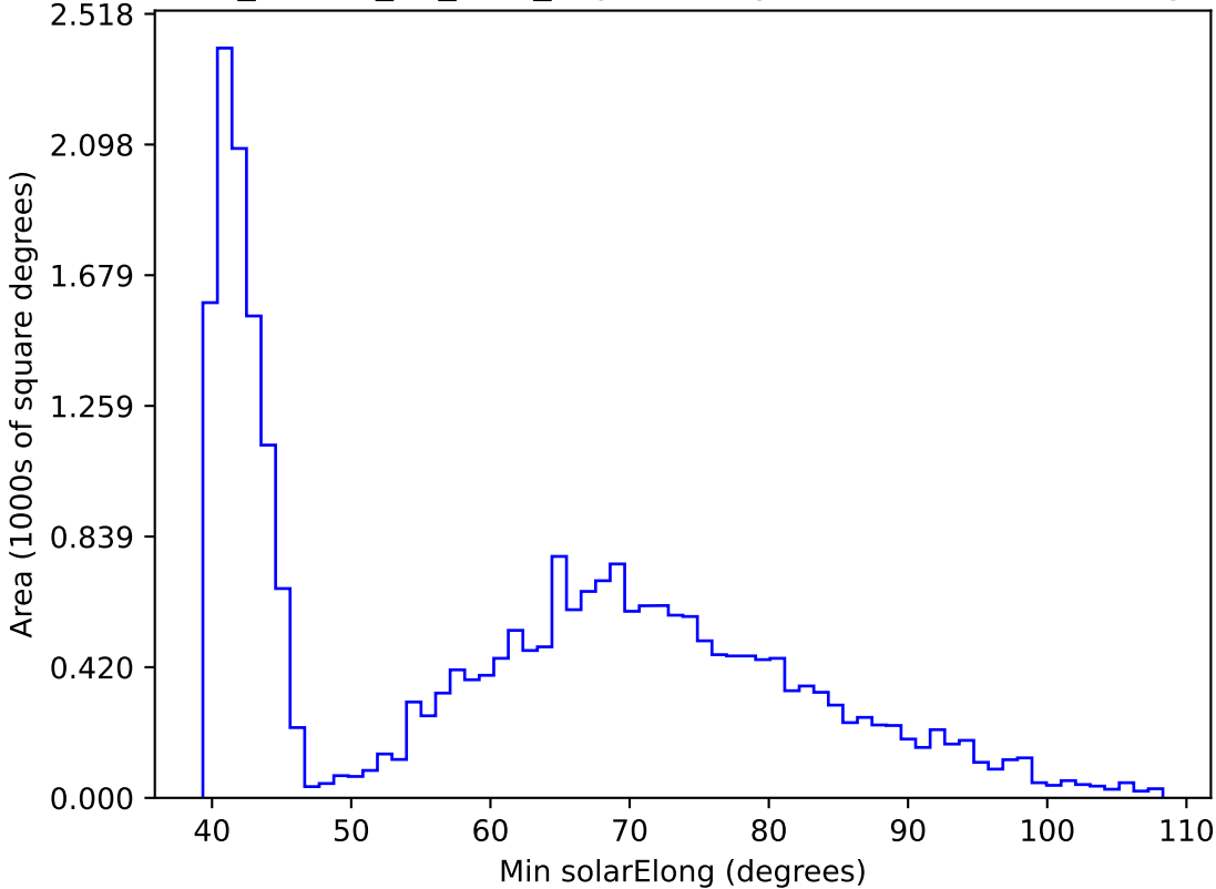
ddf_loaded_fl4_v3.4_10yrs All sky r band: Min solarElong
