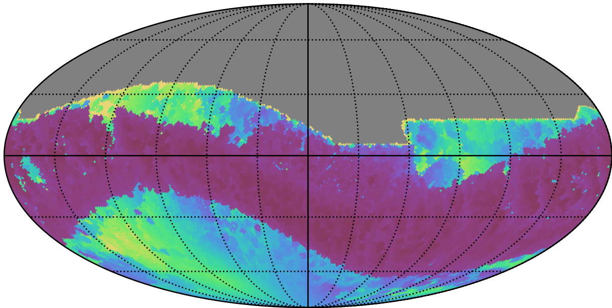
ddf_loaded_fl4_v3.4_10yrs All sky i band: Min solarElong
