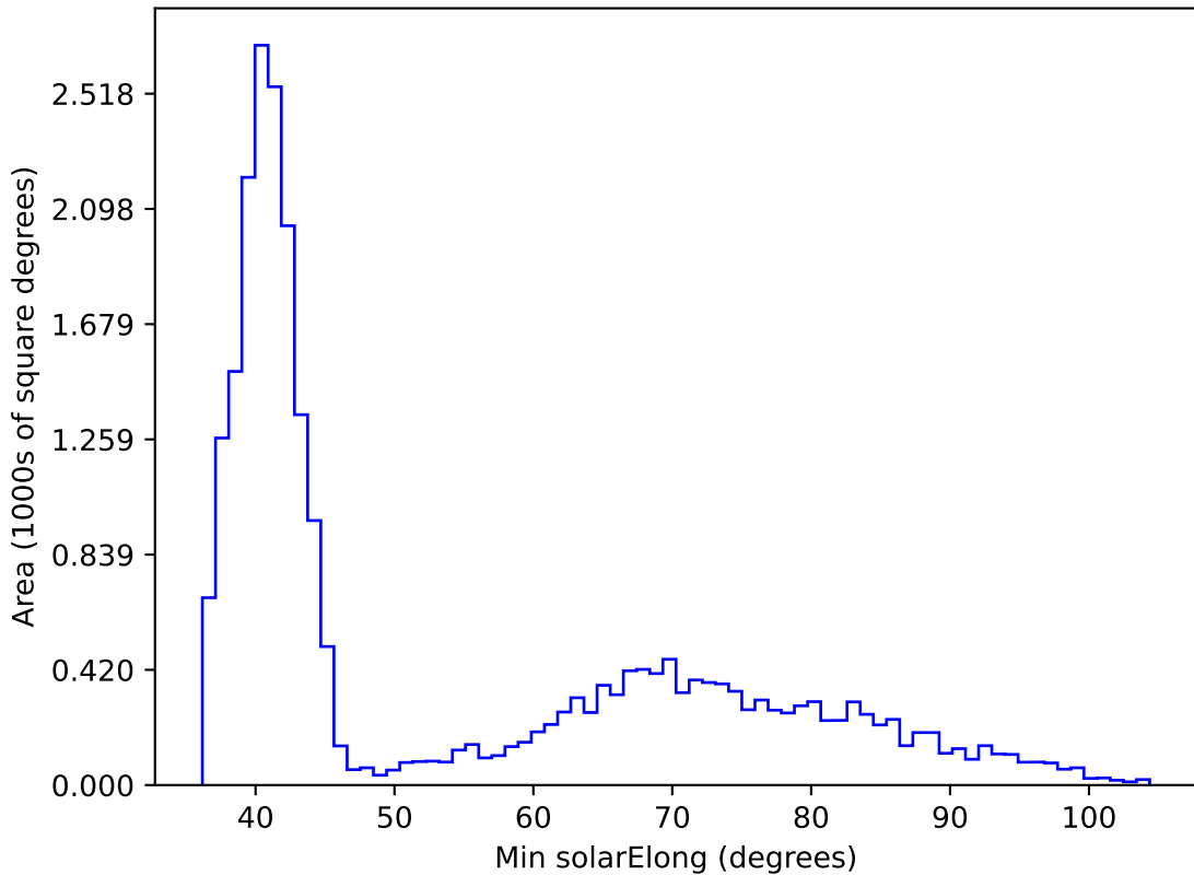
ddf_loaded_fl4_v3.4_10yrs All sky i band: Min solarElong
