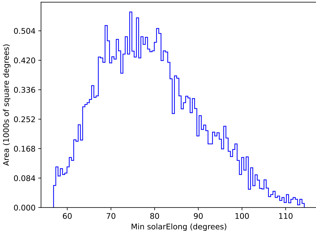
ddf_loaded_fl4_v3.4_10yrs All sky g band: Min solarElong
