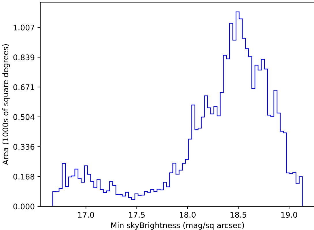
ddf_loaded_fl4_v3.4_10yrs Yr 1 z band: Min skyBrightness
