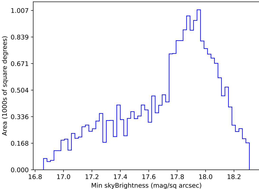
ddf_loaded_fl4_v3.4_10yrs Yr 1 y band: Min skyBrightness
