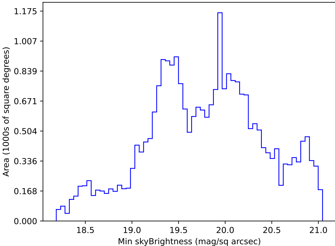
ddf_loaded_fl4_v3.4_10yrs Yr 1 r band: Min skyBrightness
