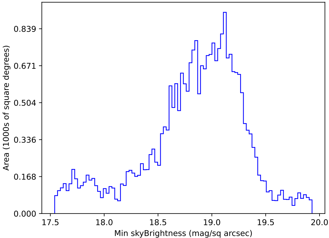
ddf_loaded_fl4_v3.4_10yrs Yr 1 i band: Min skyBrightness
