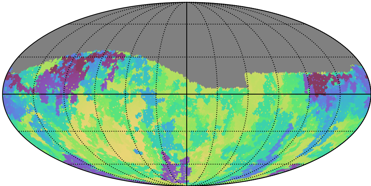
ddf_loaded_fl4_v3.4_10yrs Yr 1 g band: Min skyBrightness
