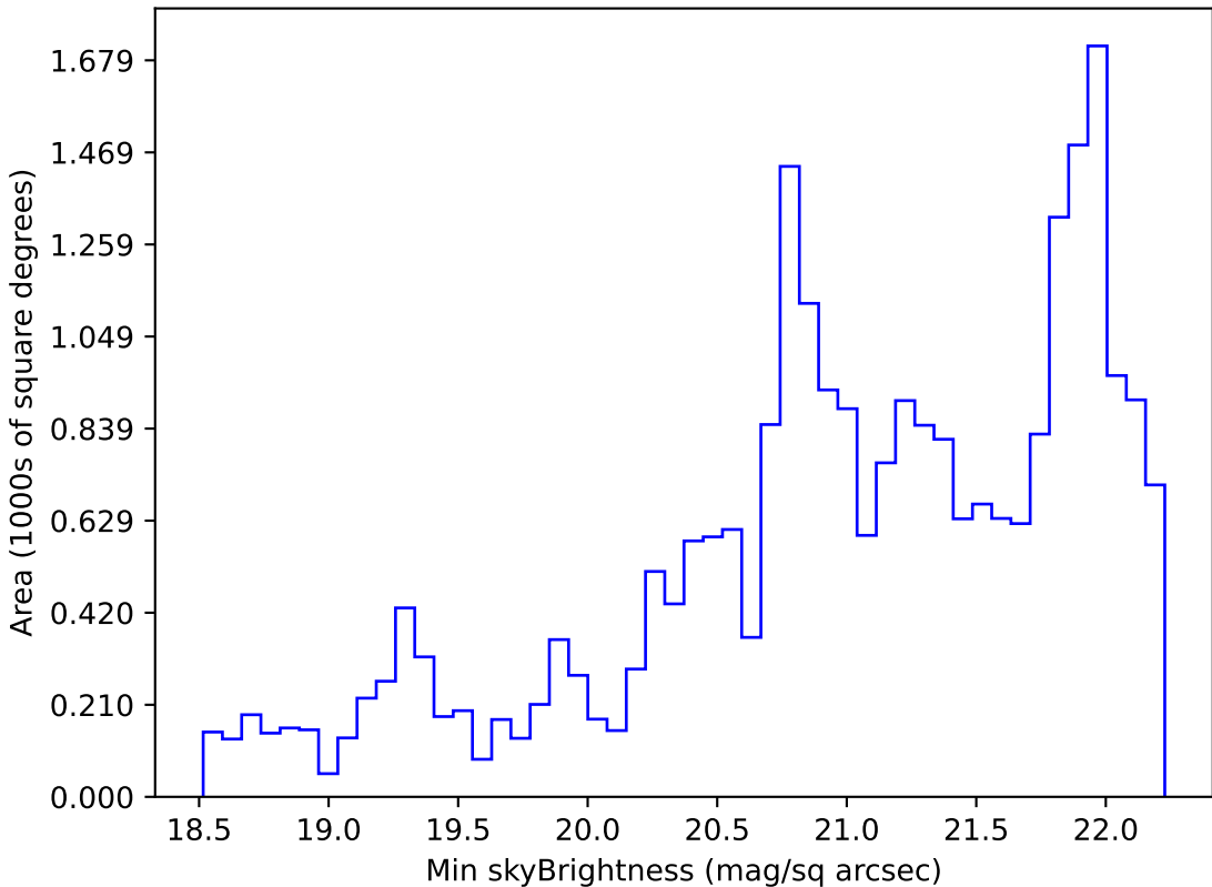
ddf_loaded_fl4_v3.4_10yrs Yr 1 g band: Min skyBrightness
