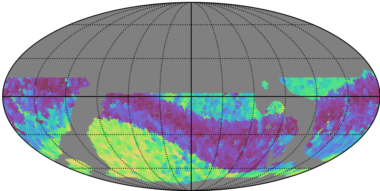
ddf_loaded_fl4_v3.4_10yrs WFD z band: Min skyBrightness
