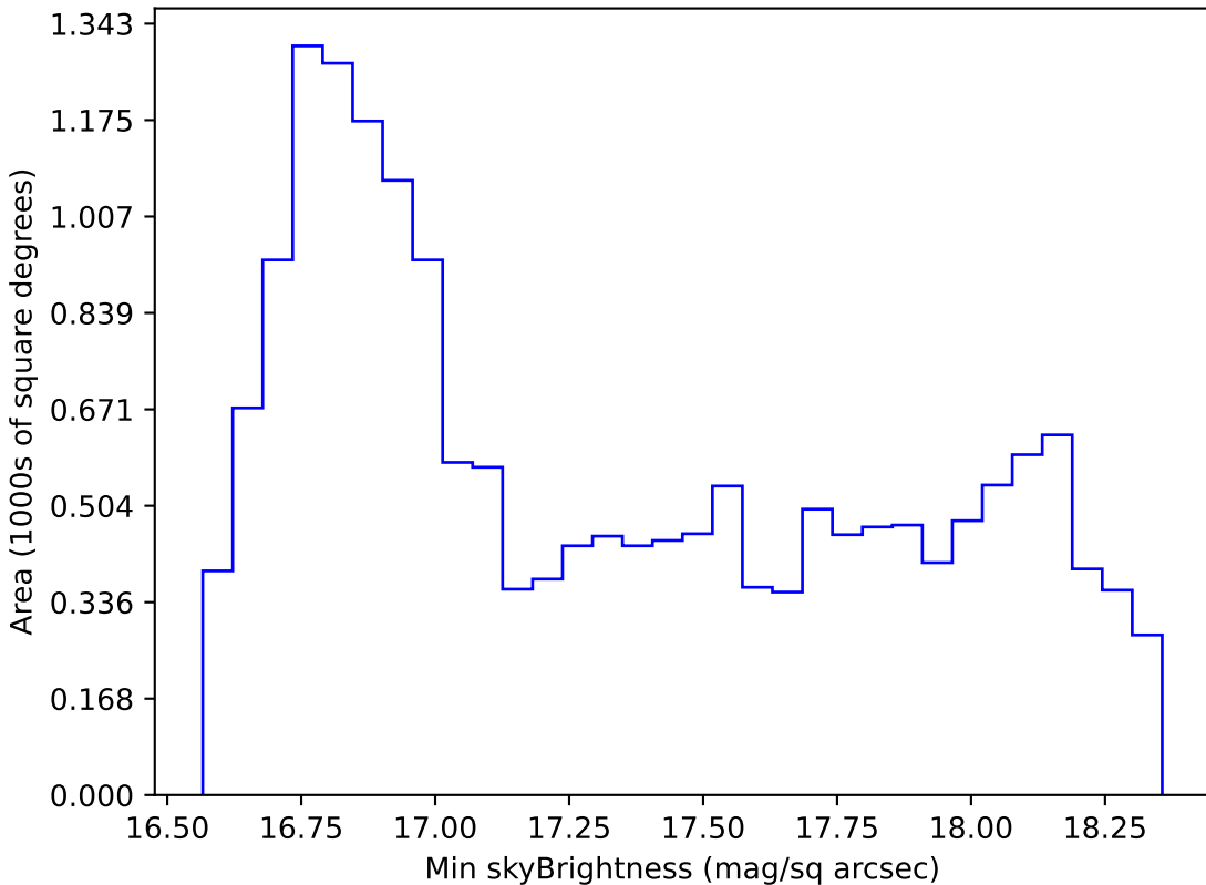
ddf_loaded_fl4_v3.4_10yrs WFD z band: Min skyBrightness
