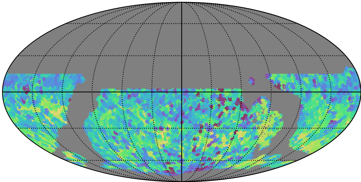
ddf_loaded_fl4_v3.4_10yrs WFD y band: Min skyBrightness
