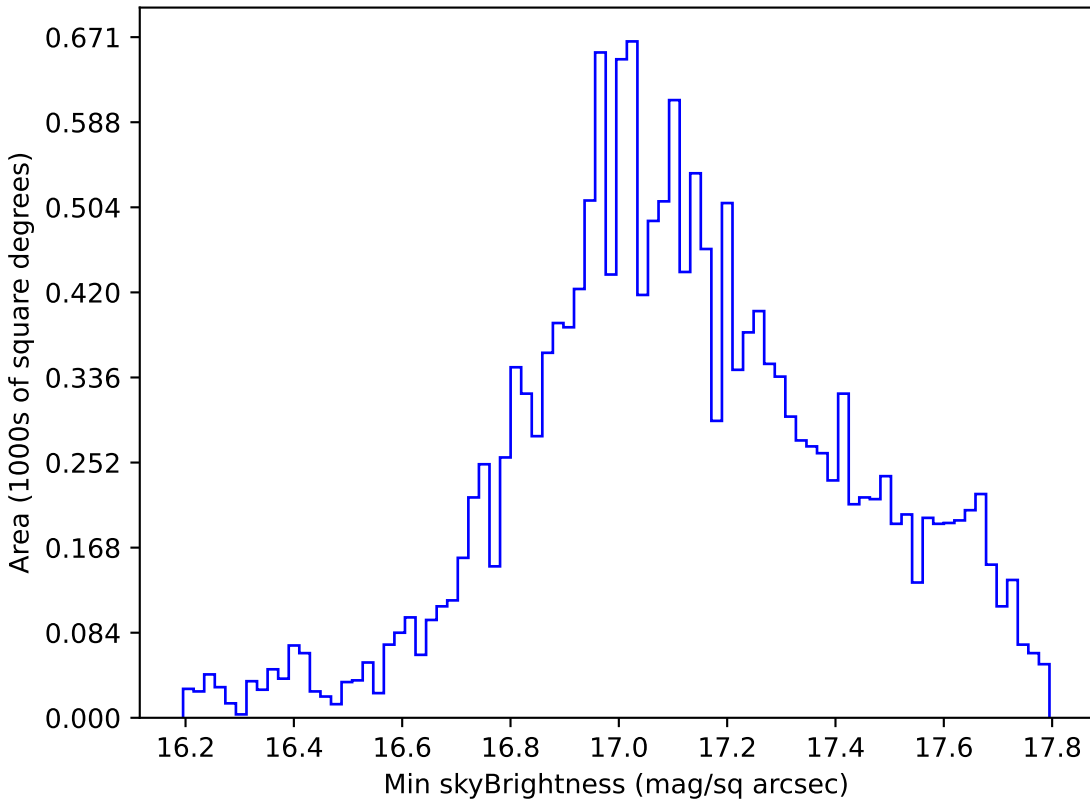
ddf_loaded_fl4_v3.4_10yrs WFD y band: Min skyBrightness
