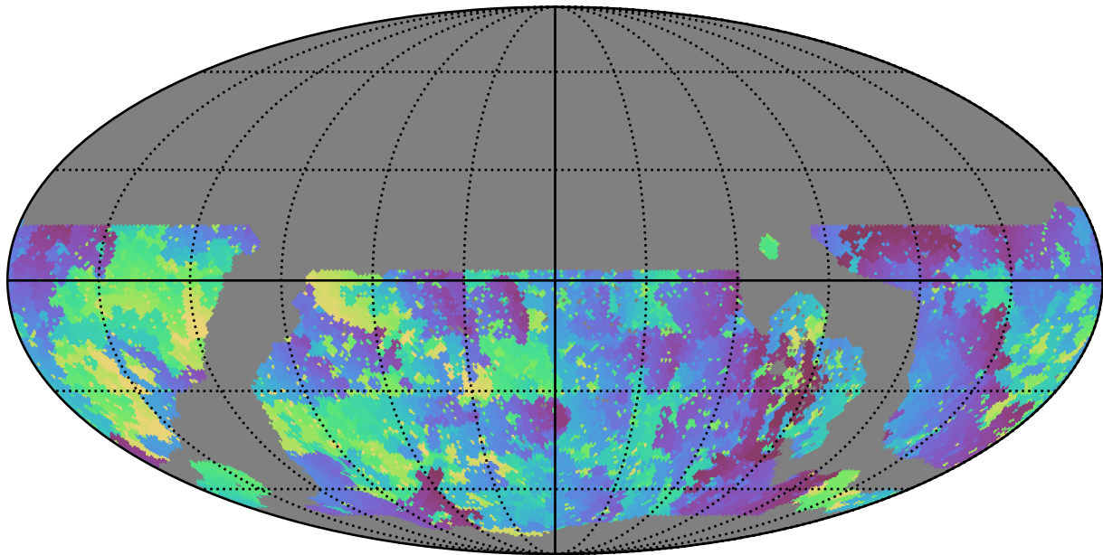
ddf_loaded_fl4_v3.4_10yrs WFD u band: Min skyBrightness
