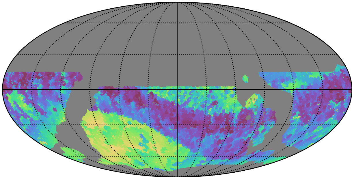
ddf_loaded_fl4_v3.4_10yrs WFD i band: Min skyBrightness
