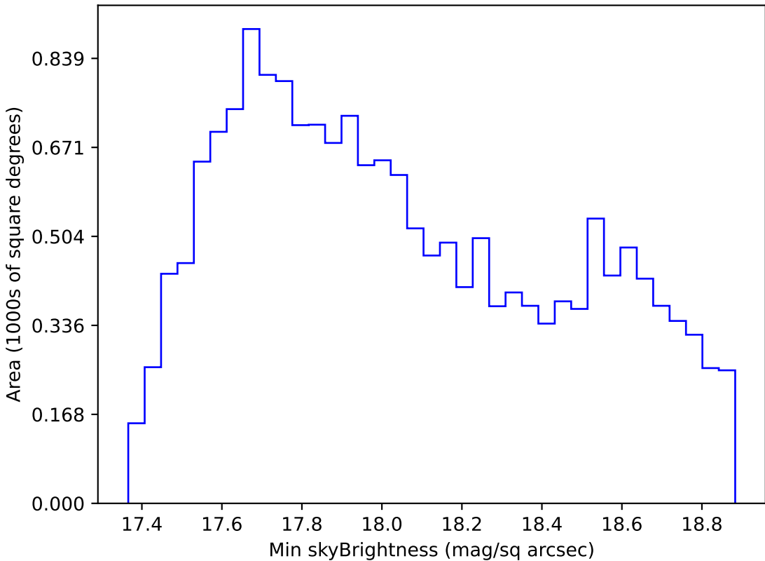
ddf_loaded_fl4_v3.4_10yrs WFD i band: Min skyBrightness
