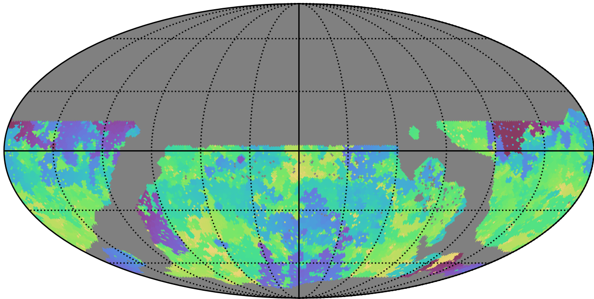
ddf_loaded_fl4_v3.4_10yrs WFD g band: Min skyBrightness
