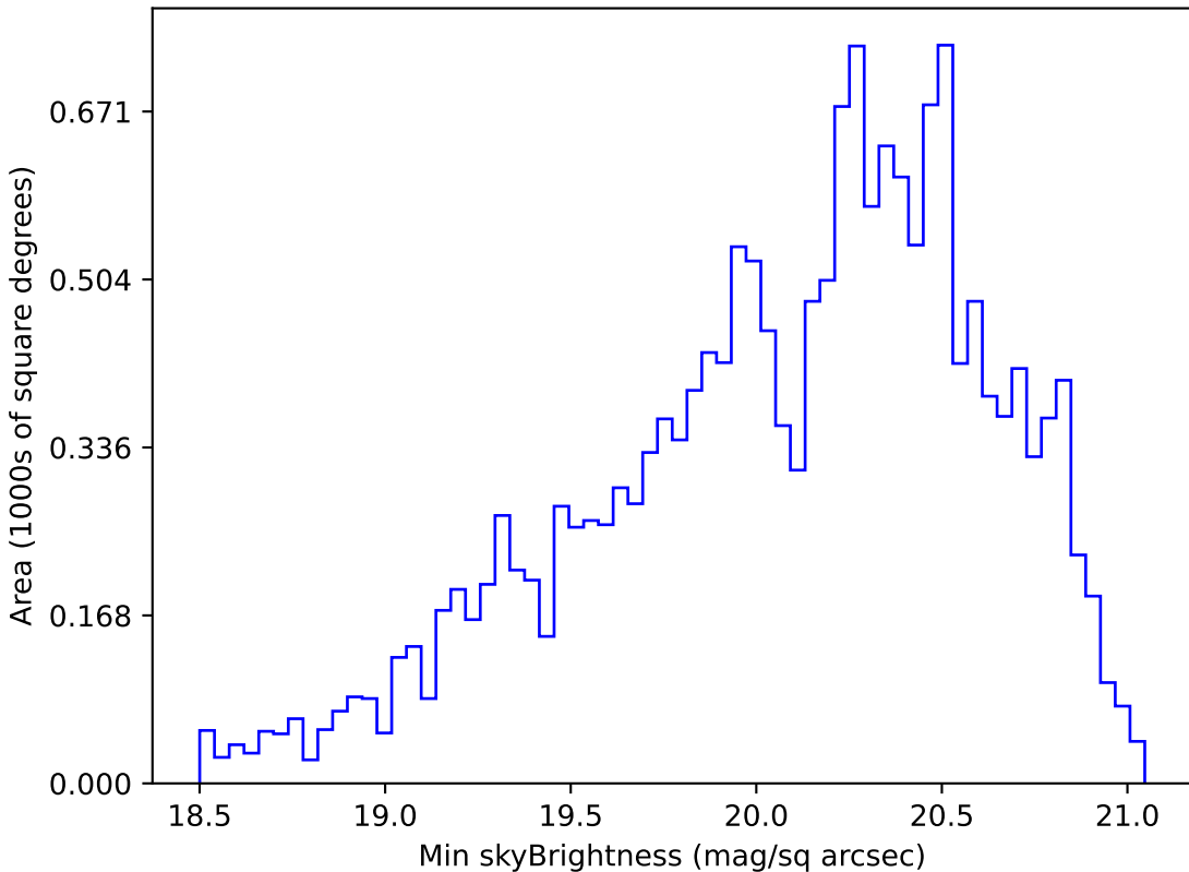
ddf_loaded_fl4_v3.4_10yrs WFD g band: Min skyBrightness
