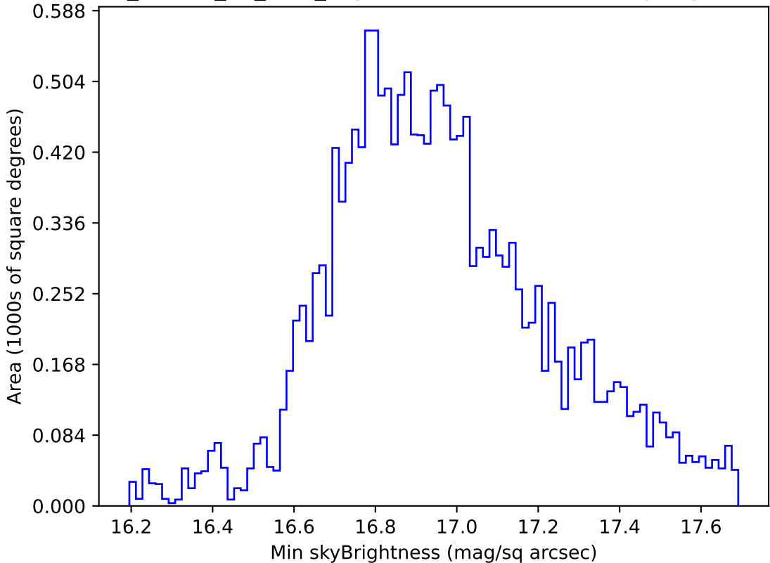
ddf_loaded_fl4_v3.4_10yrs WFD all bands: Min skyBrightness
