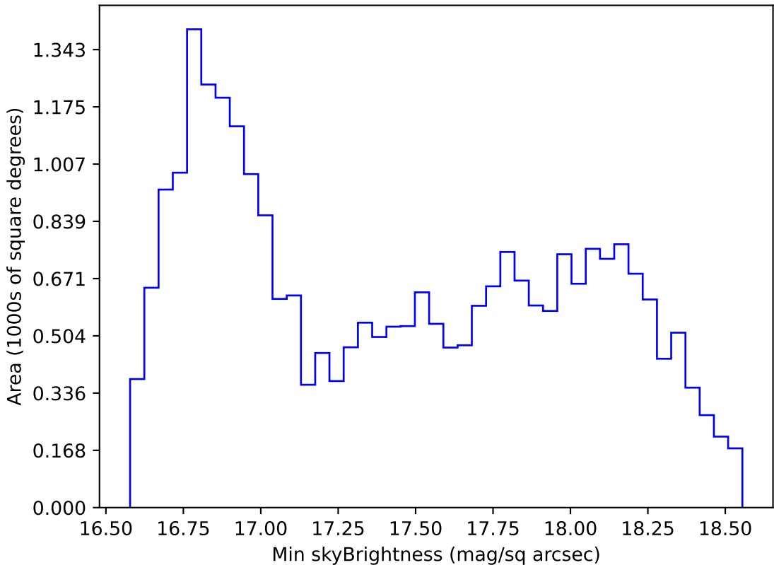
ddf_loaded_fl4_v3.4_10yrs All sky z band: Min skyBrightness
