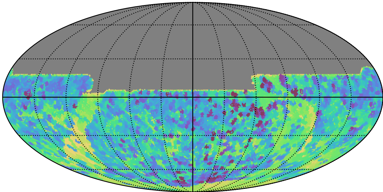
ddf_loaded_fl4_v3.4_10yrs All sky y band: Min skyBrightness
