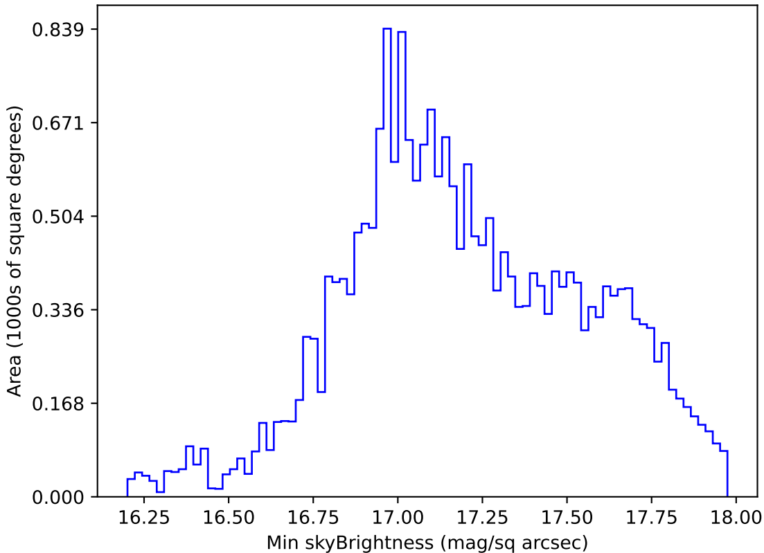
ddf_loaded_fl4_v3.4_10yrs All sky y band: Min skyBrightness
