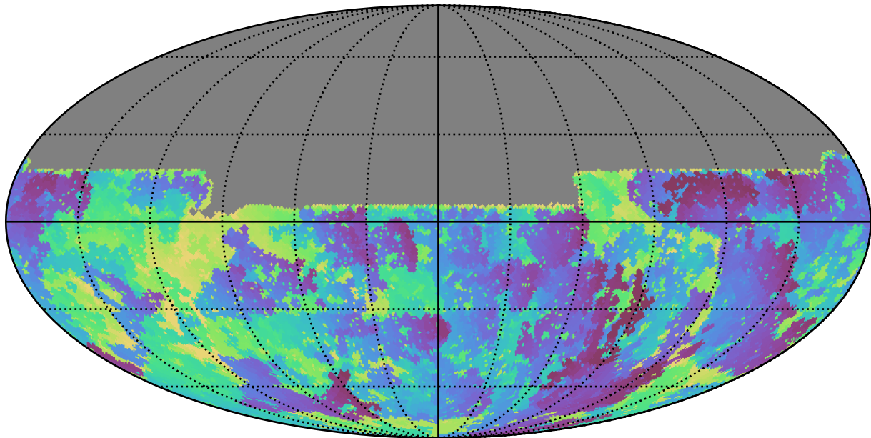
ddf_loaded_fl4_v3.4_10yrs All sky u band: Min skyBrightness
