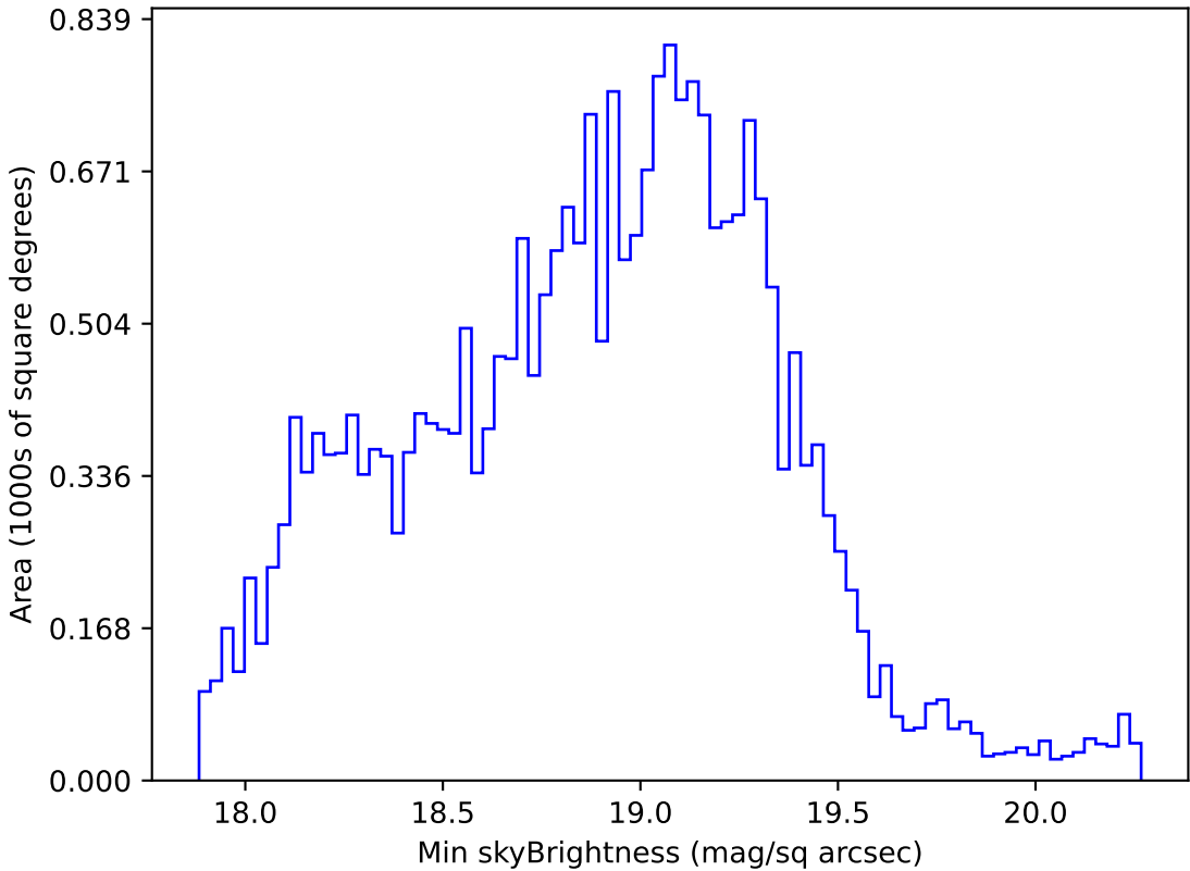
ddf_loaded_fl4_v3.4_10yrs All sky r band: Min skyBrightness
