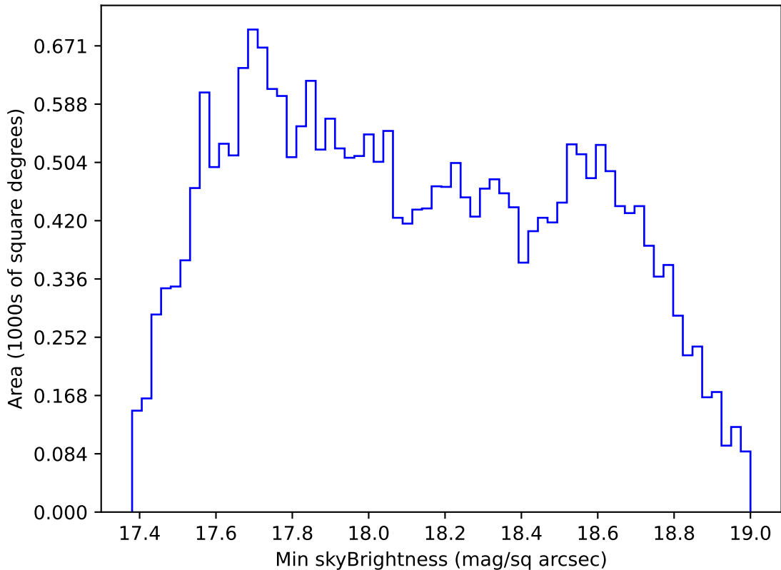
ddf_loaded_fl4_v3.4_10yrs All sky i band: Min skyBrightness
