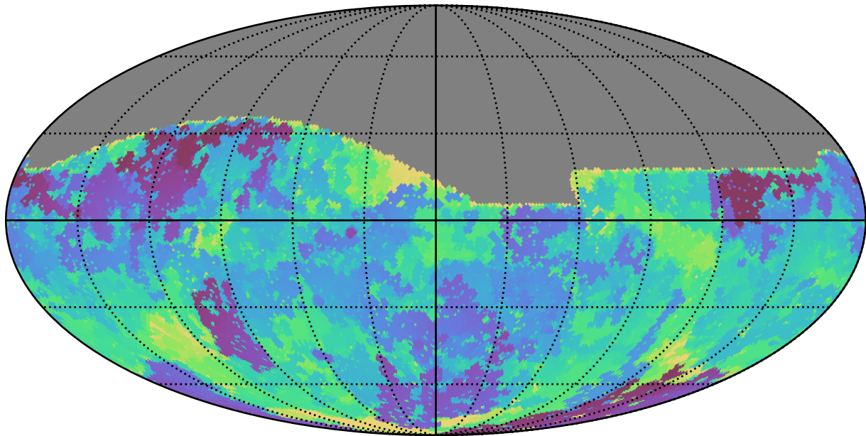
ddf_loaded_fl4_v3.4_10yrs All sky g band: Min skyBrightness
