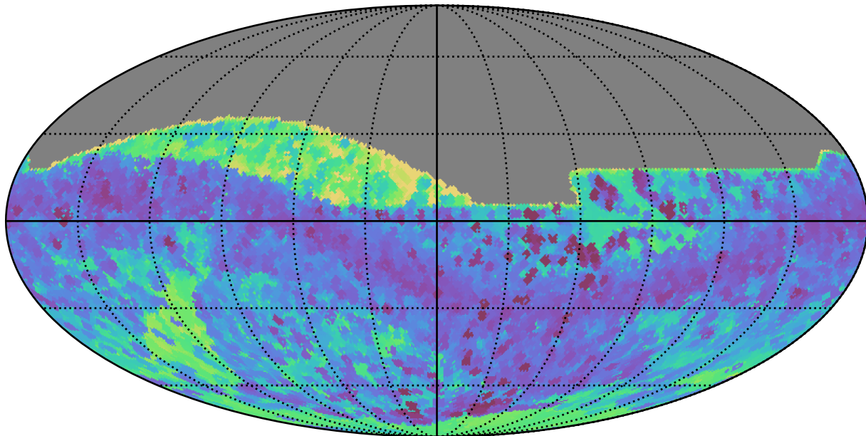
ddf_loaded_fl4_v3.4_10yrs All sky all bands: Min skyBrightness
