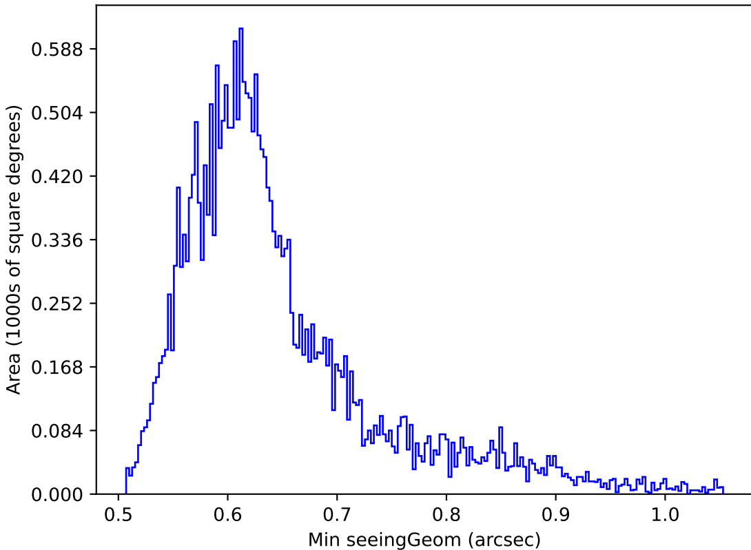
ddf_loaded_fl4_v3.4_10yrs Yr 1 z band: Min seeingGeom
