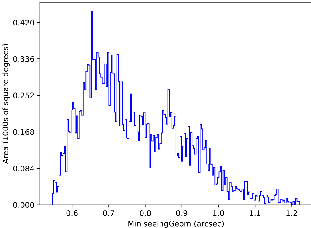
ddf_loaded_fl4_v3.4_10yrs Yr 1 u band: Min seeingGeom
