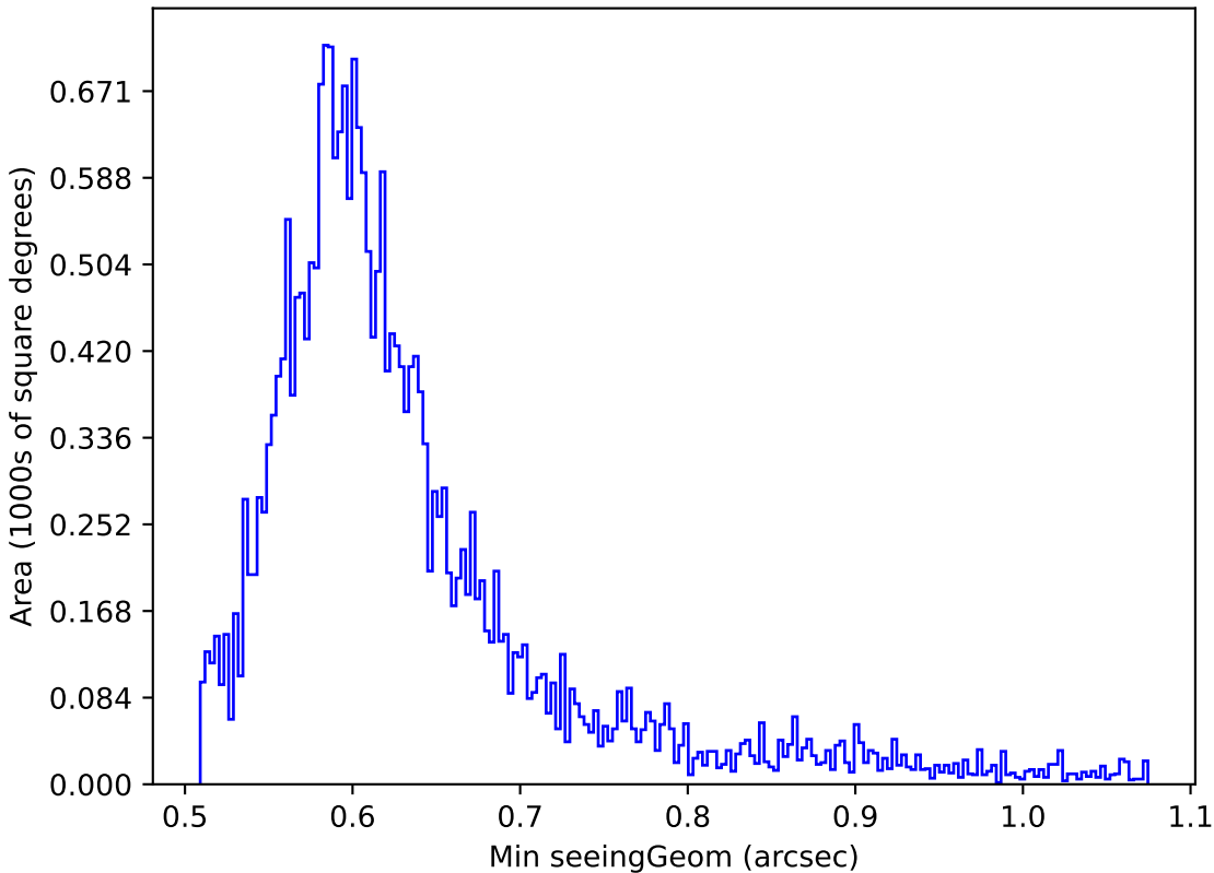
ddf_loaded_fl4_v3.4_10yrs Yr 1 i band: Min seeingGeom
