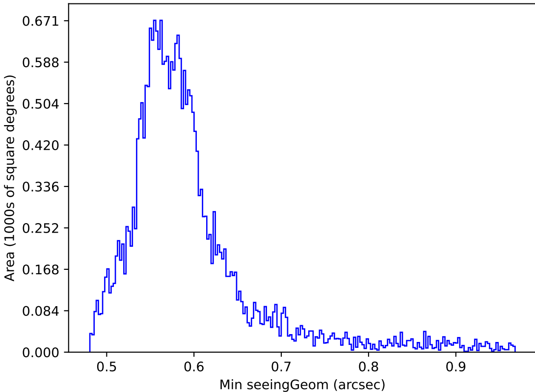
ddf_loaded_fl4_v3.4_10yrs Yr 1 all bands: Min seeingGeom
