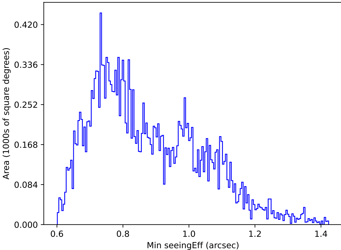
ddf_loaded_fl4_v3.4_10yrs Yr 1 u band: Min seeingEff
