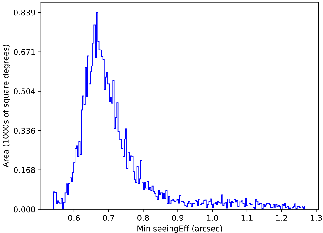
ddf_loaded_fl4_v3.4_10yrs Yr 1 r band: Min seeingEff
