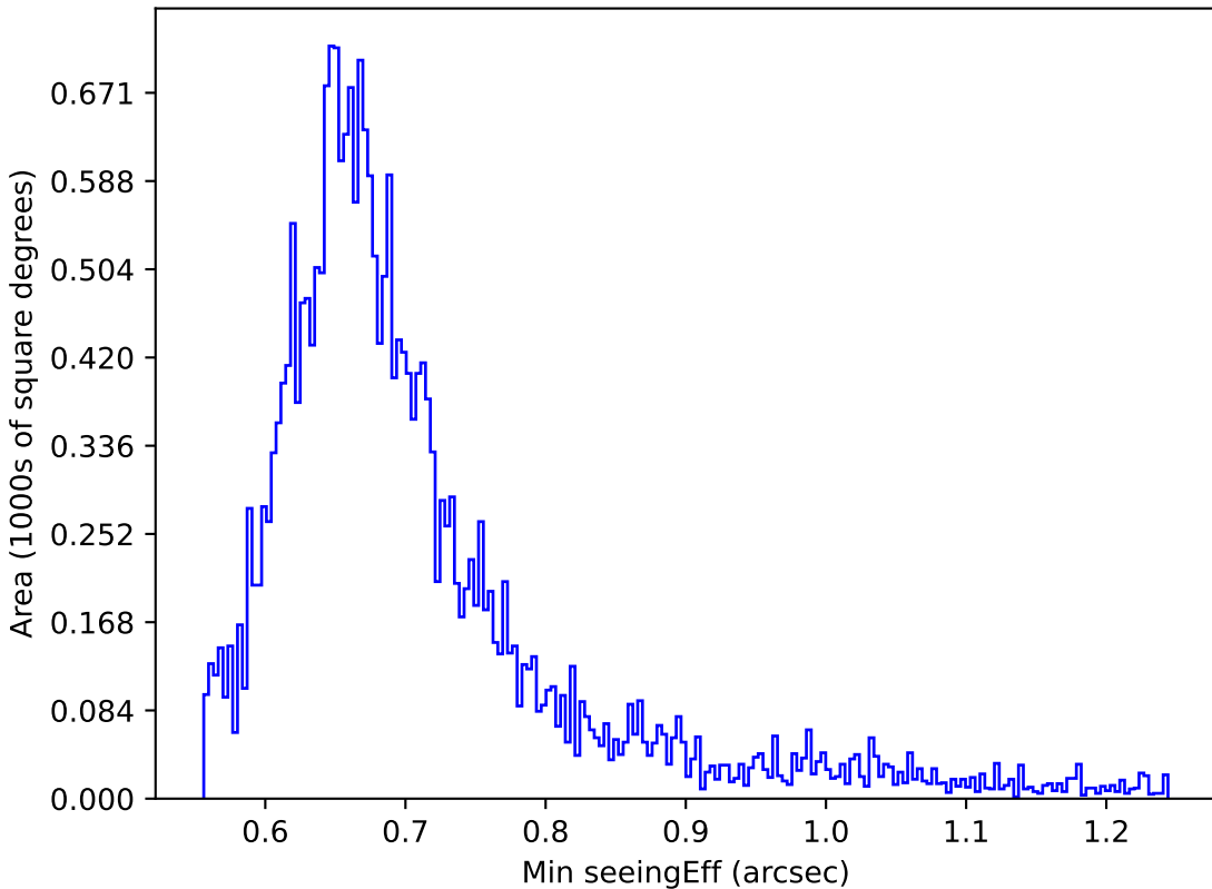
ddf_loaded_fl4_v3.4_10yrs Yr 1 i band: Min seeingEff
