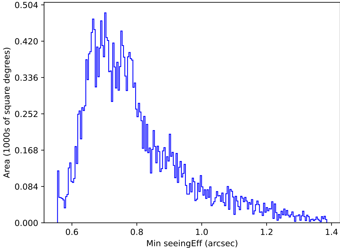
ddf_loaded_fl4_v3.4_10yrs Yr 1 g band: Min seeingEff
