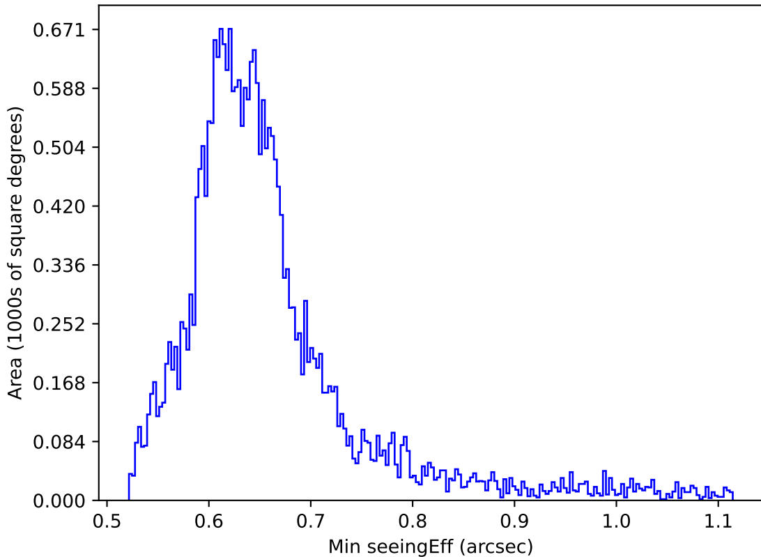
ddf_loaded_fl4_v3.4_10yrs Yr 1 all bands: Min seeingEff
