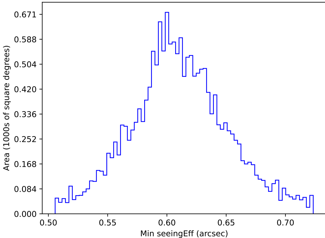
ddf_loaded_fl4_v3.4_10yrs WFD z band: Min seeingEff
