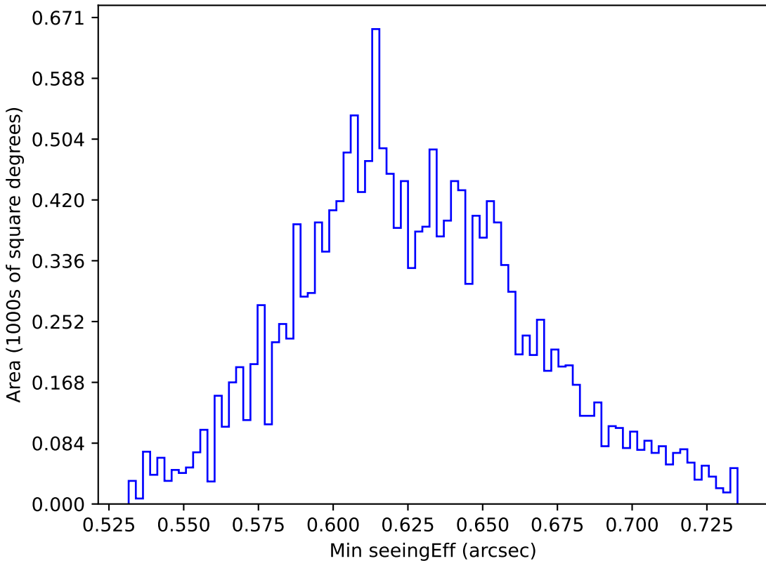
ddf_loaded_fl4_v3.4_10yrs WFD y band: Min seeingEff
