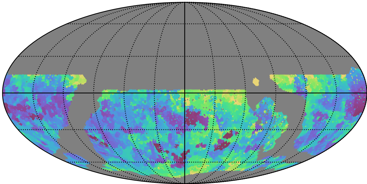
ddf_loaded_fl4_v3.4_10yrs WFD u band: Min seeingEff
