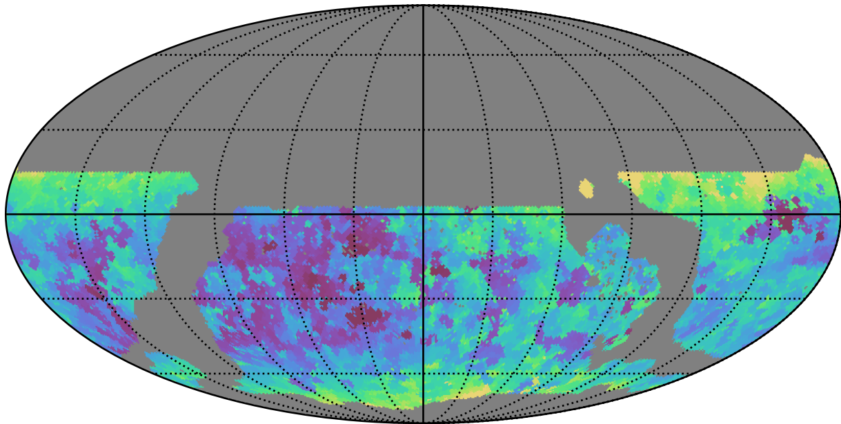
ddf_loaded_fl4_v3.4_10yrs WFD r band: Min seeingEff
