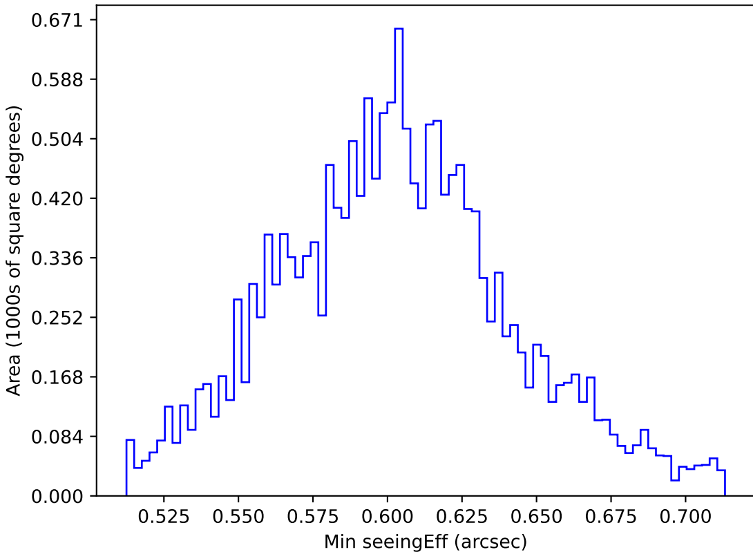
ddf_loaded_fl4_v3.4_10yrs WFD i band: Min seeingEff
