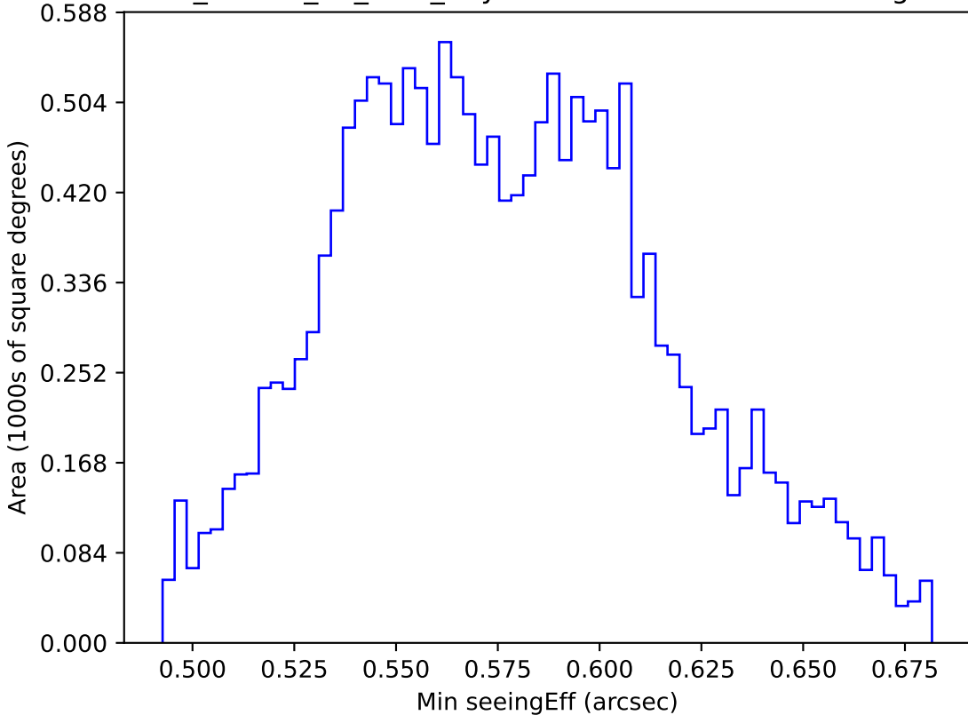
ddf_loaded_fl4_v3.4_10yrs WFD all bands: Min seeingEff
