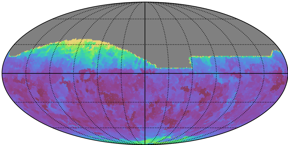
ddf_loaded_fl4_v3.4_10yrs All sky z band: Min seeingEff
