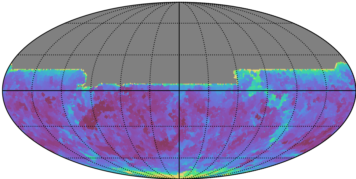
ddf_loaded_fl4_v3.4_10yrs All sky y band: Min seeingEff
