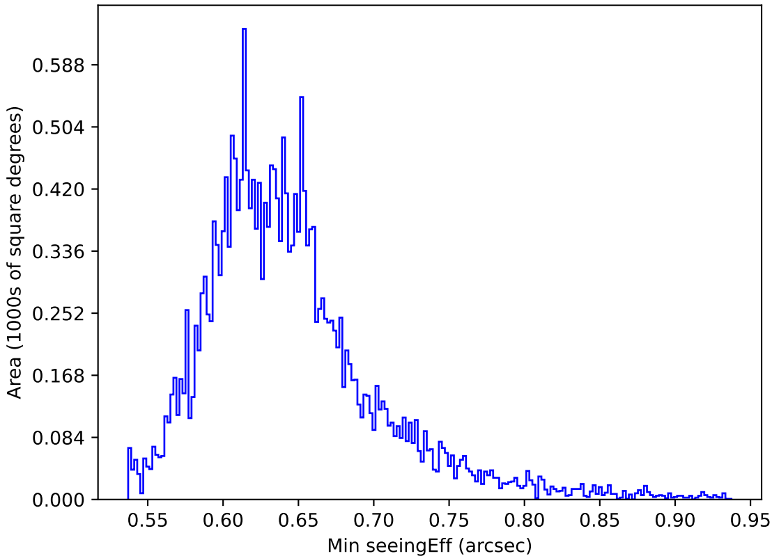
ddf_loaded_fl4_v3.4_10yrs All sky y band: Min seeingEff
