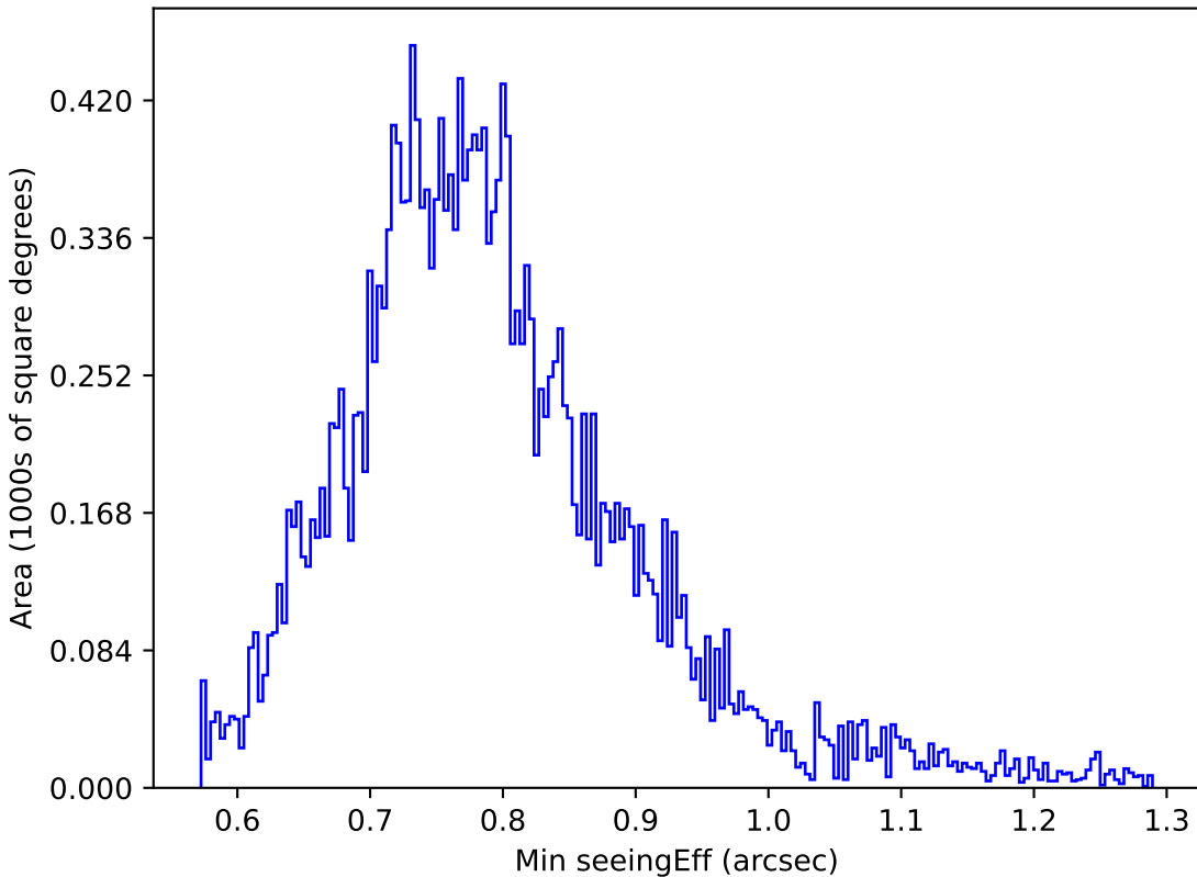
ddf_loaded_fl4_v3.4_10yrs All sky u band: Min seeingEff
