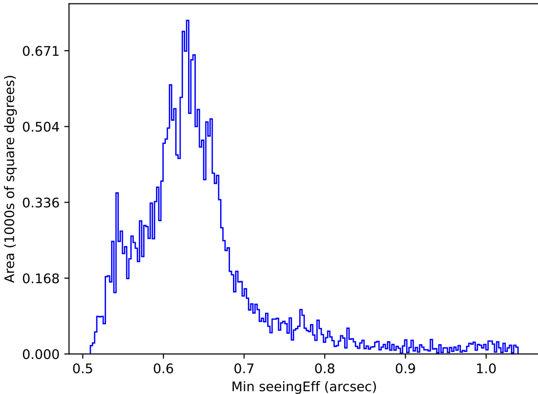
ddf_loaded_fl4_v3.4_10yrs All sky r band: Min seeingEff
